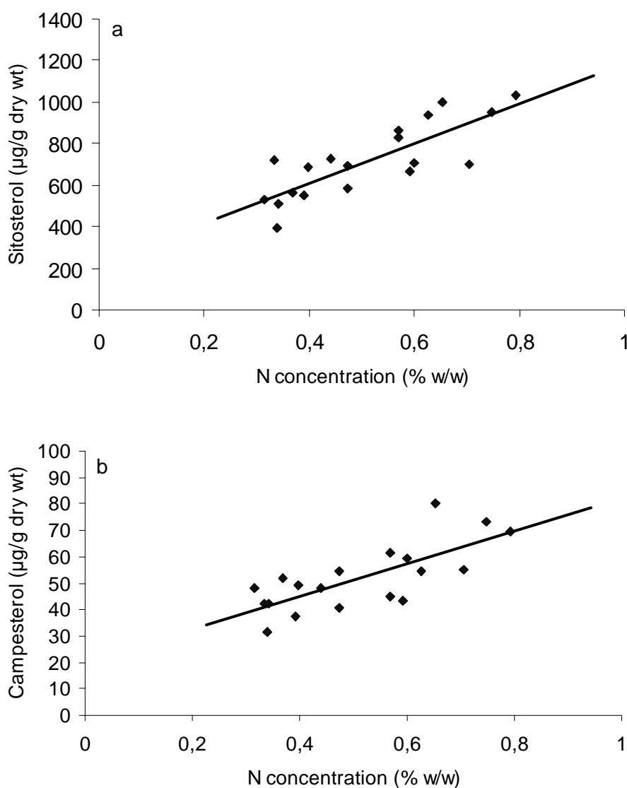
Fig. 3.4 Regression between N concentration (% w/w) and (a) sitosterol content, and (b) campesterol content (µg/g dry weight) in shoots of Plantago lanceolata
